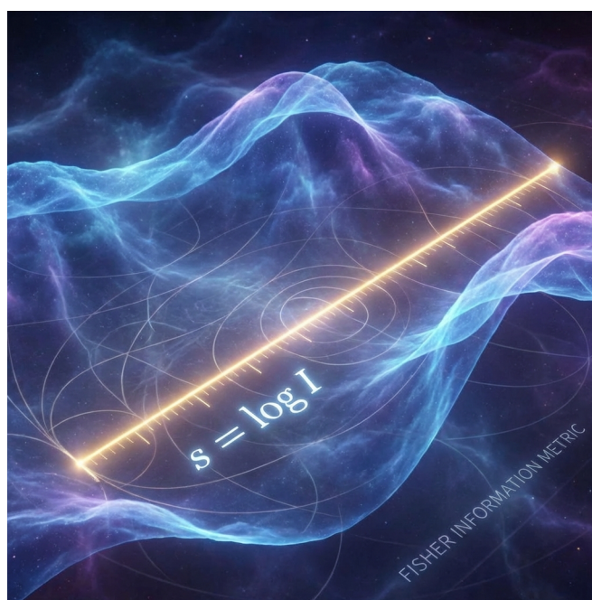
Figure B.1: Fisher Manifold
