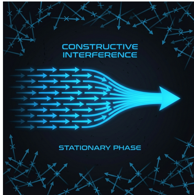
Figure 2.2: Stationary Phase
