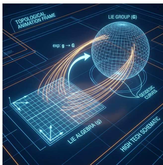
Figure C.1: Lie Wrapping
