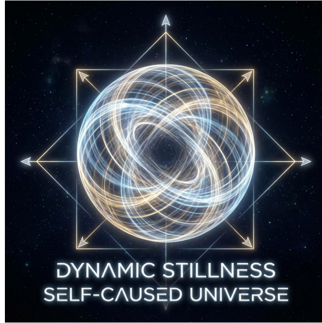
Figure 9.3: Ultimate State
