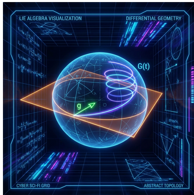
Figure 3.2: Lie Algebra Tangent
