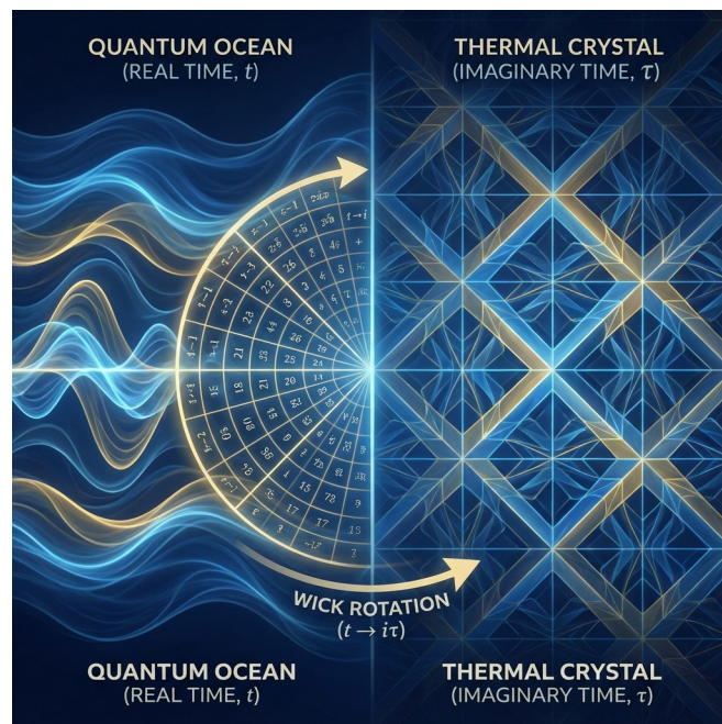
Figure 5.1: Wick Rotation
