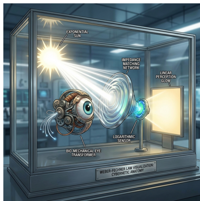
Figure 8.1: Weber Eye
