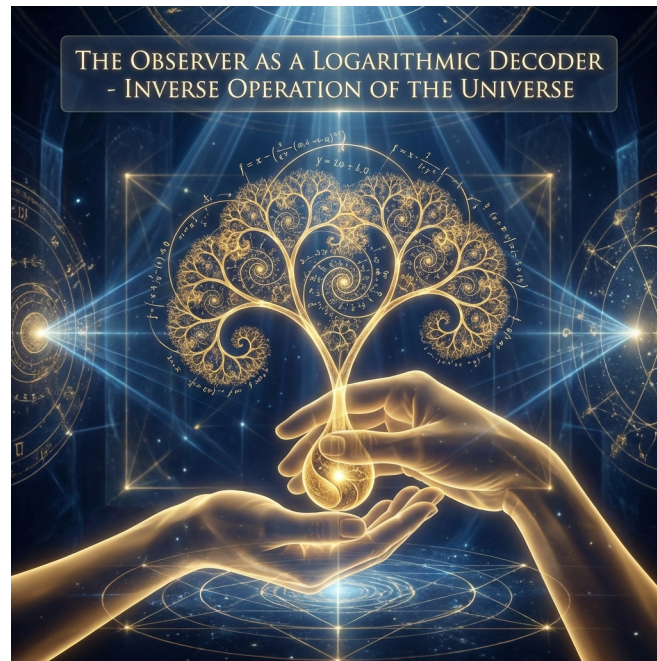
Figure 7.2: Observer Decoder
