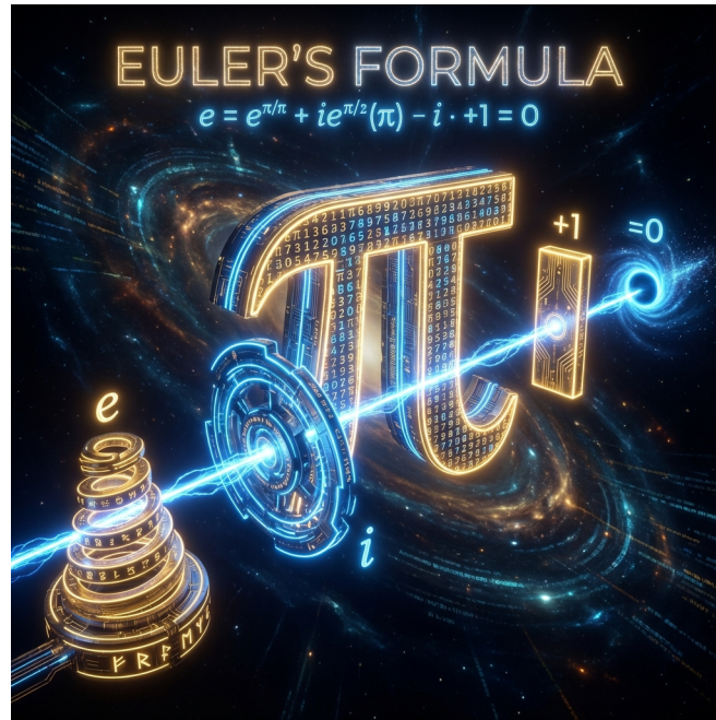
Figure 1: Euler's Map
