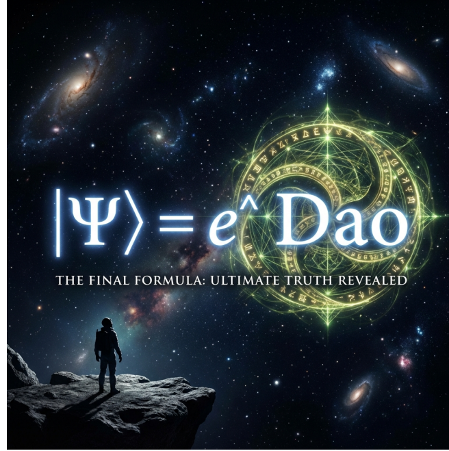
Figure 9.2: Final Formula
