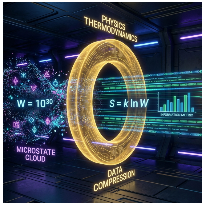
Figure 7.1: Boltzmann Logarithm
